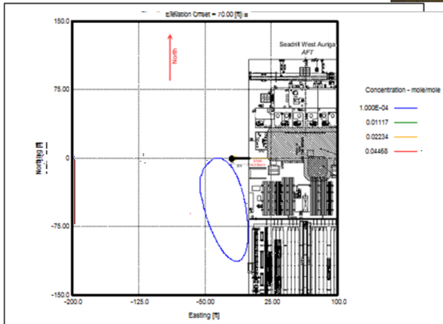
Figure 14 – Gas concentrations for Vent Case 4 – wind -15 deg from North Elevation @ 70 ft
